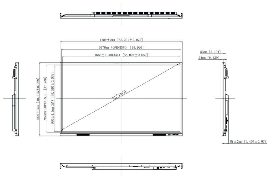
75" : ST-75-UHD-AND-HP-007-S
