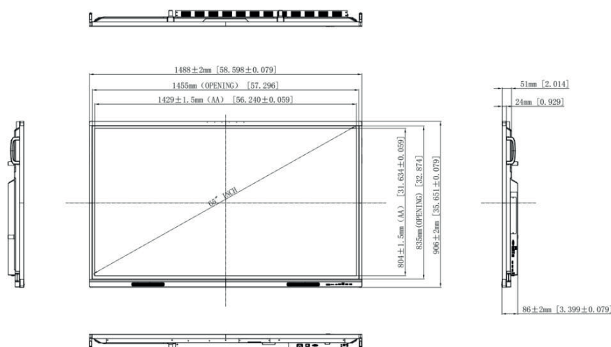
65" : ST-65-UHD-AND-HP-007-S
